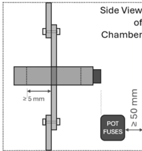
Figure 4 - CT Chamber general dimensions
