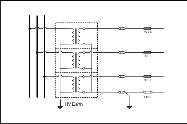
Figure 6 - Star Point Earth (3-phase Cat B VT)
