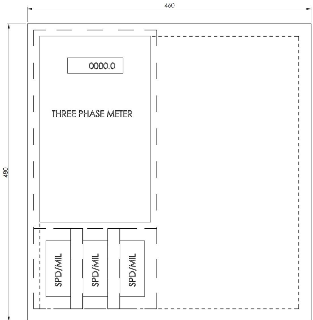
Figure 20 - Typical Panel Layout for Residential House with Multi-phase meter
