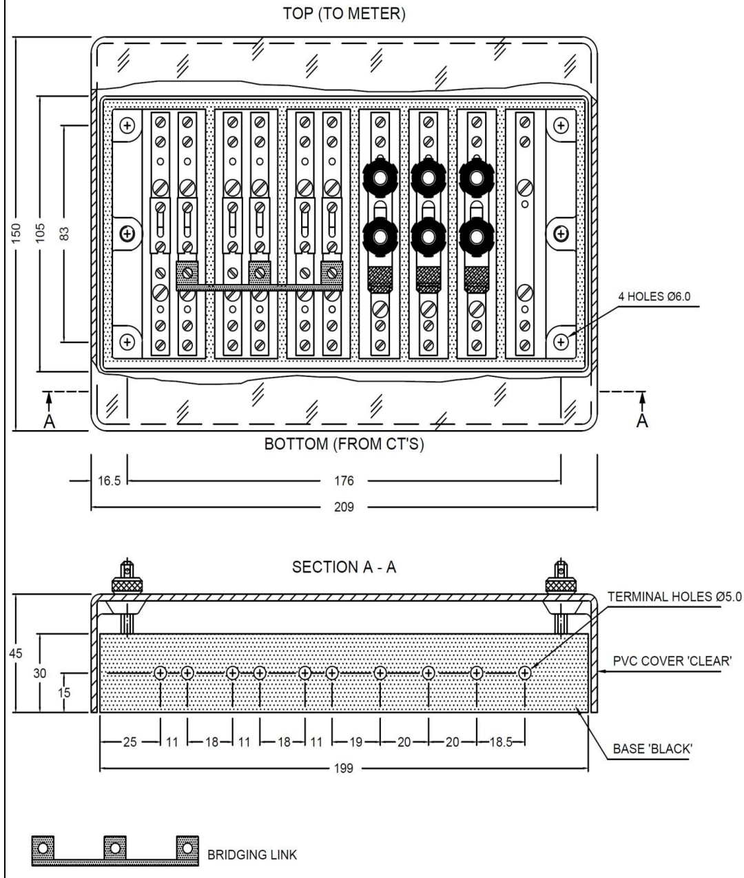
Figure 35 – Test Block Arrangement
