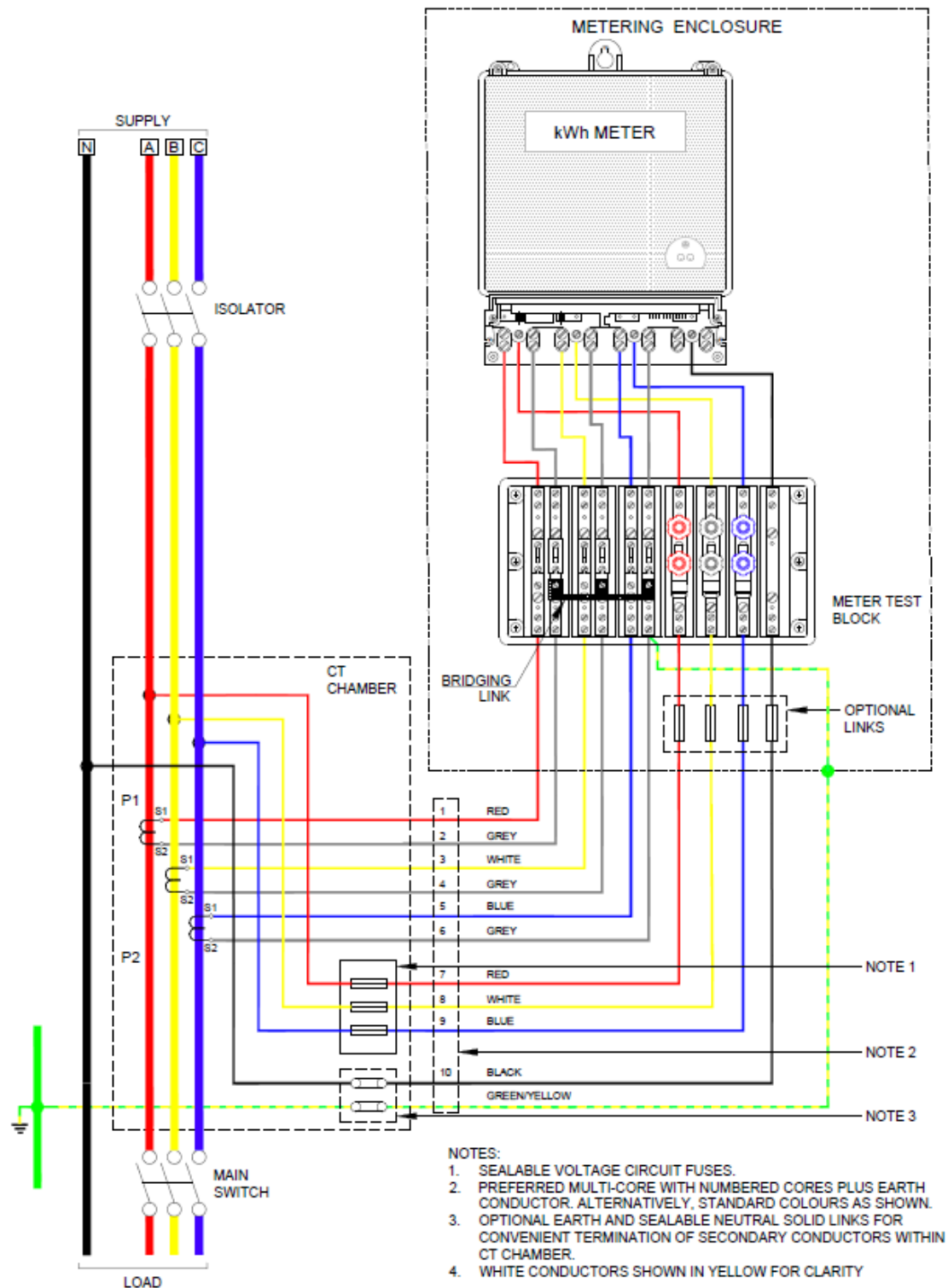
Figure 34 - Wiring Diagram for CT Metering
