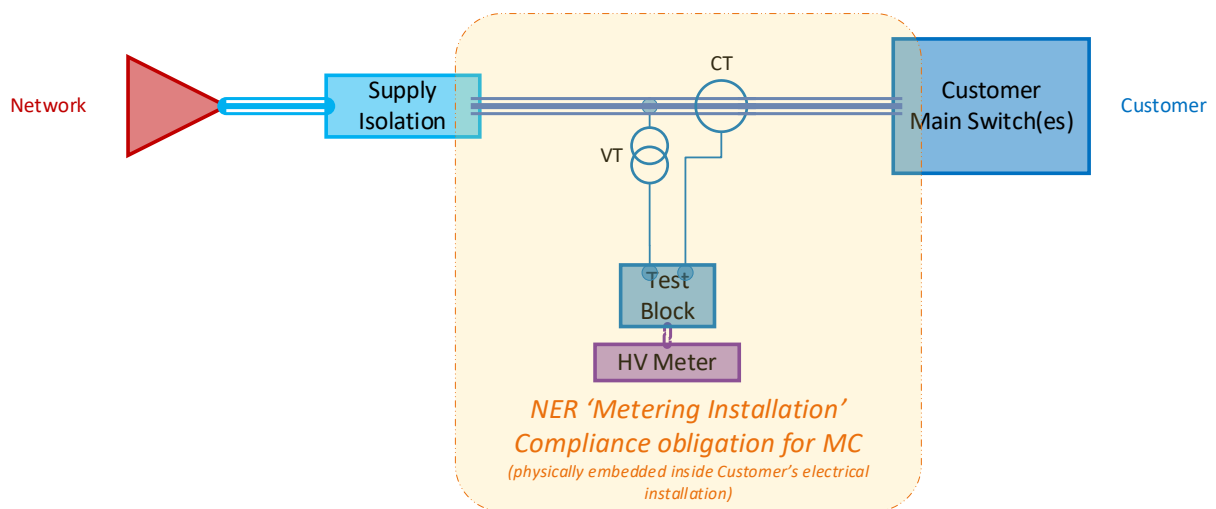
Figure 3 - HV Metering Installation Responsibilities and Ownerships
