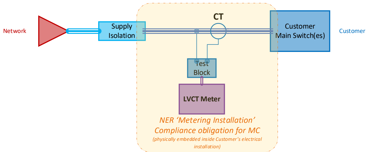
Figure 2 - LVCT Metering Installation Responsibilities and Ownerships
