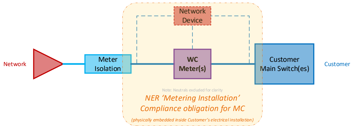
Figure 1 - WC Metering Installation Responsibilities and Ownerships
