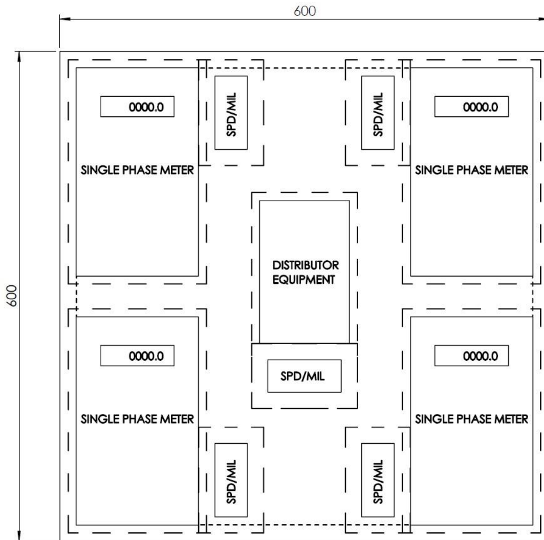
Figure 27 - Typical Panel Layout for Multi Occupancy, Single phase, 600 x 600 panel
