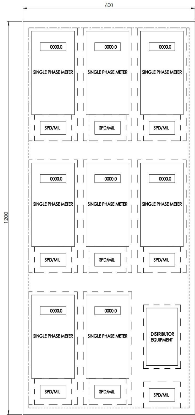
Figure 21 - Typical Panel Layout for Multi Occupancy, Single phase, 1200 x 600 panel
