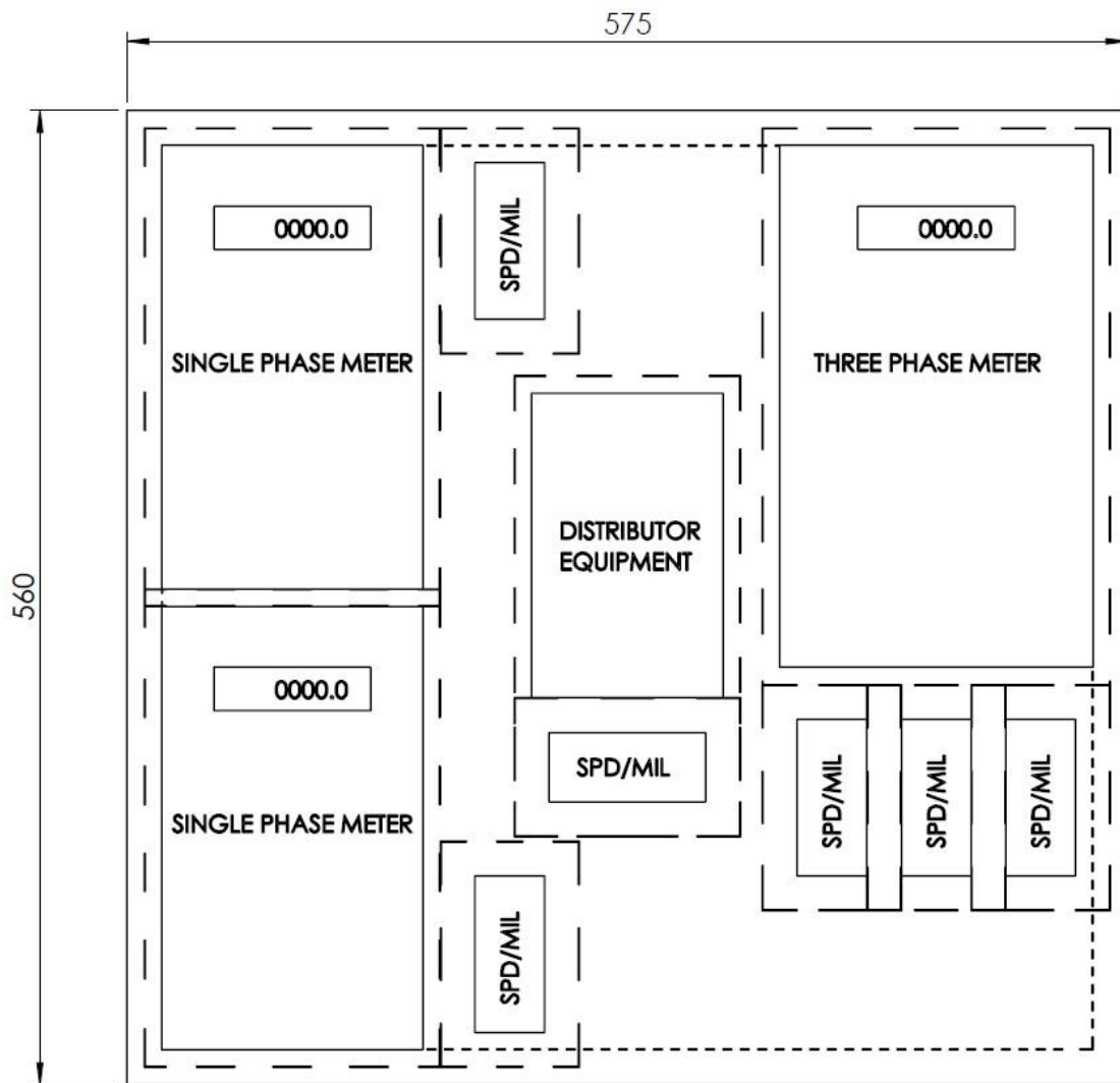
Figure 29 - Typical Panel Layout for Multi Occupancy, multiphase and single phase, 560 x 575 panel
