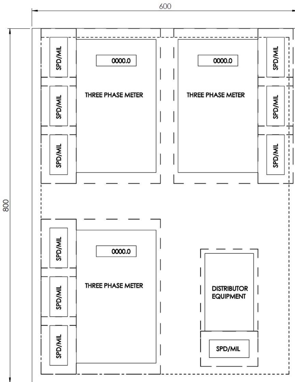
Figure 26 - Typical Panel Layout for Multi Occupancy, multiphase, 800 x 600 panel
