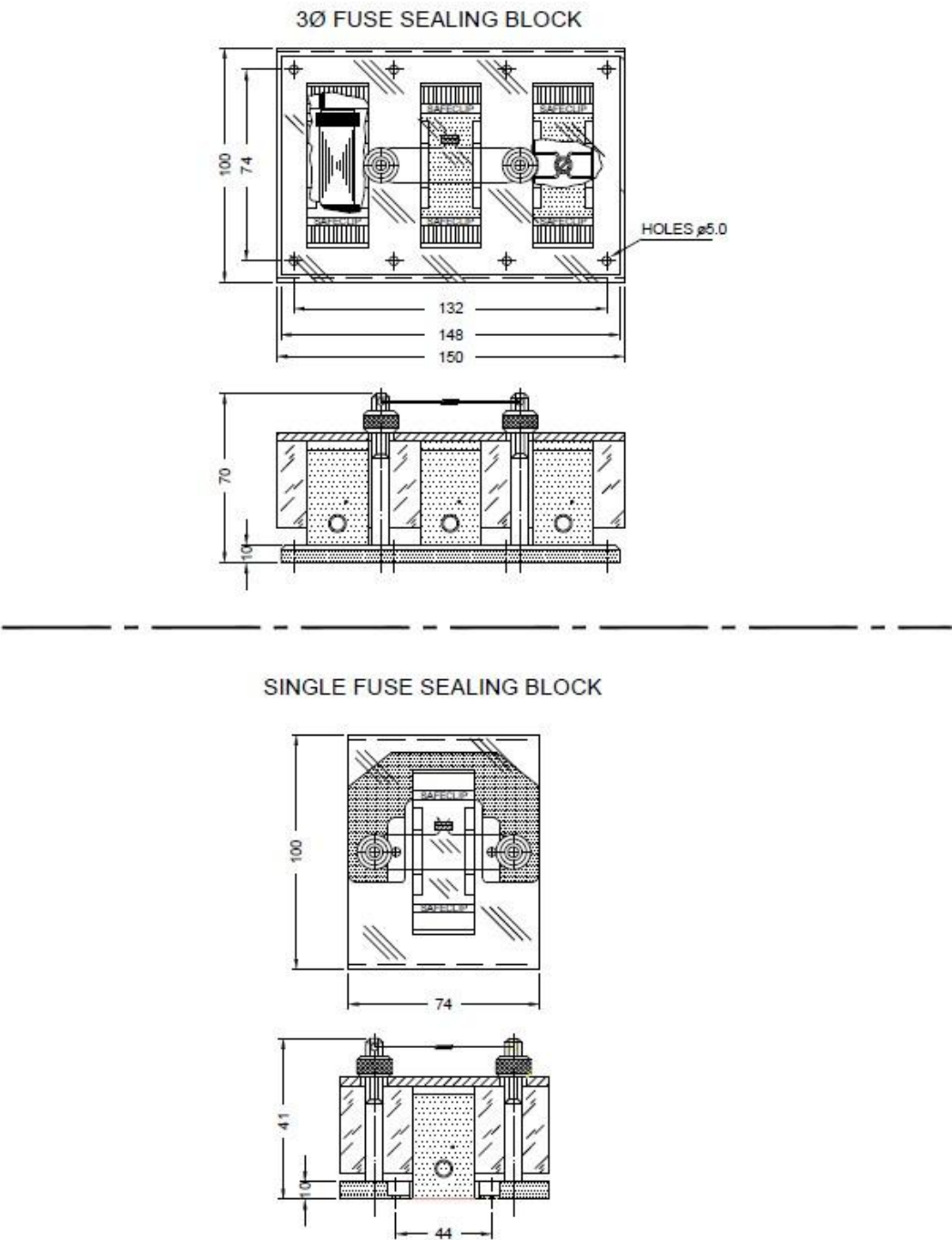
Figure 31 - General arrangement for metering fuse sealing blocks
