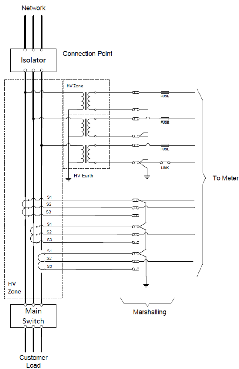
Figure 5 - Metering Arrangement with CTs and VT Star Point Earth (3 x single phase VT's)
