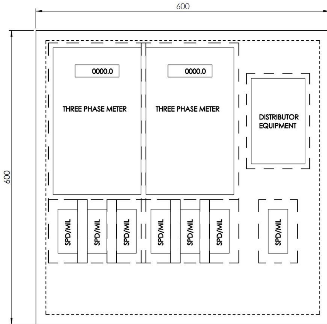
Figure 28- Typical Panel Layout for Multi Occupancy, multiphase, 600 x 600 panel
