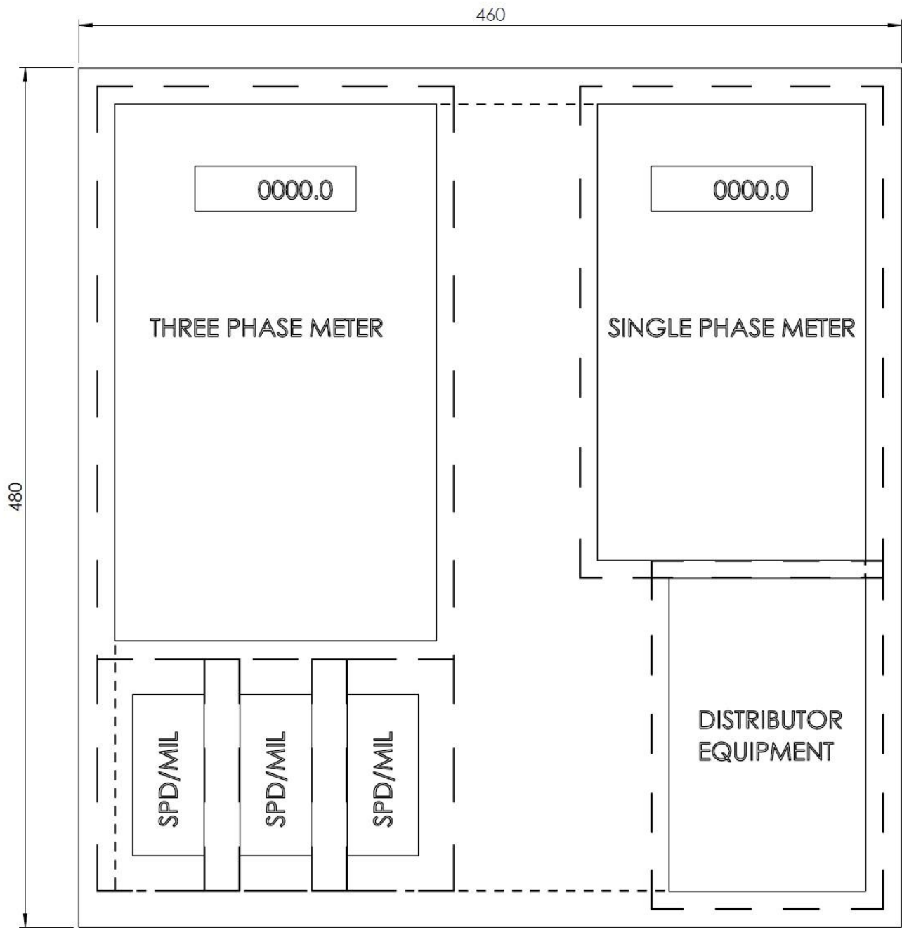
Figure 19 - Typical Panel Layout for Residential House with Multi-phase, single phase meters and load control
