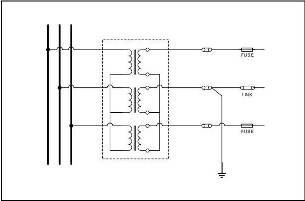
Figure 7 - Reference Polarity Earth (3-phase Cat A VT)
