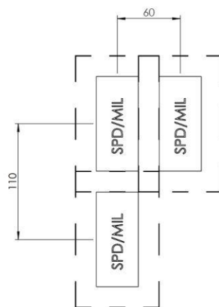
Figure 11 - Meter Protection / Isolation Devices
