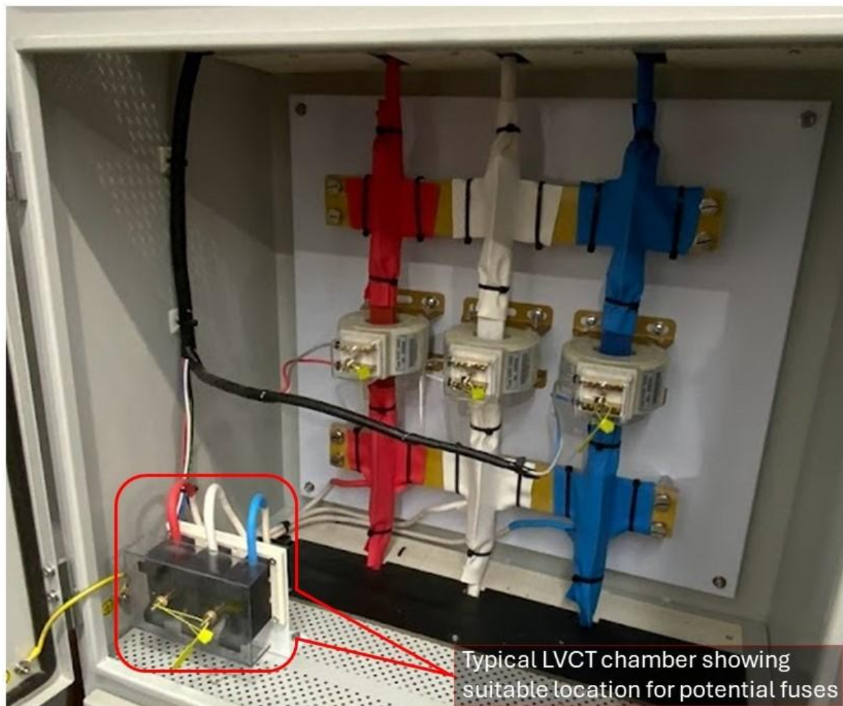
Figure 33 –LVCT chamber Photo
