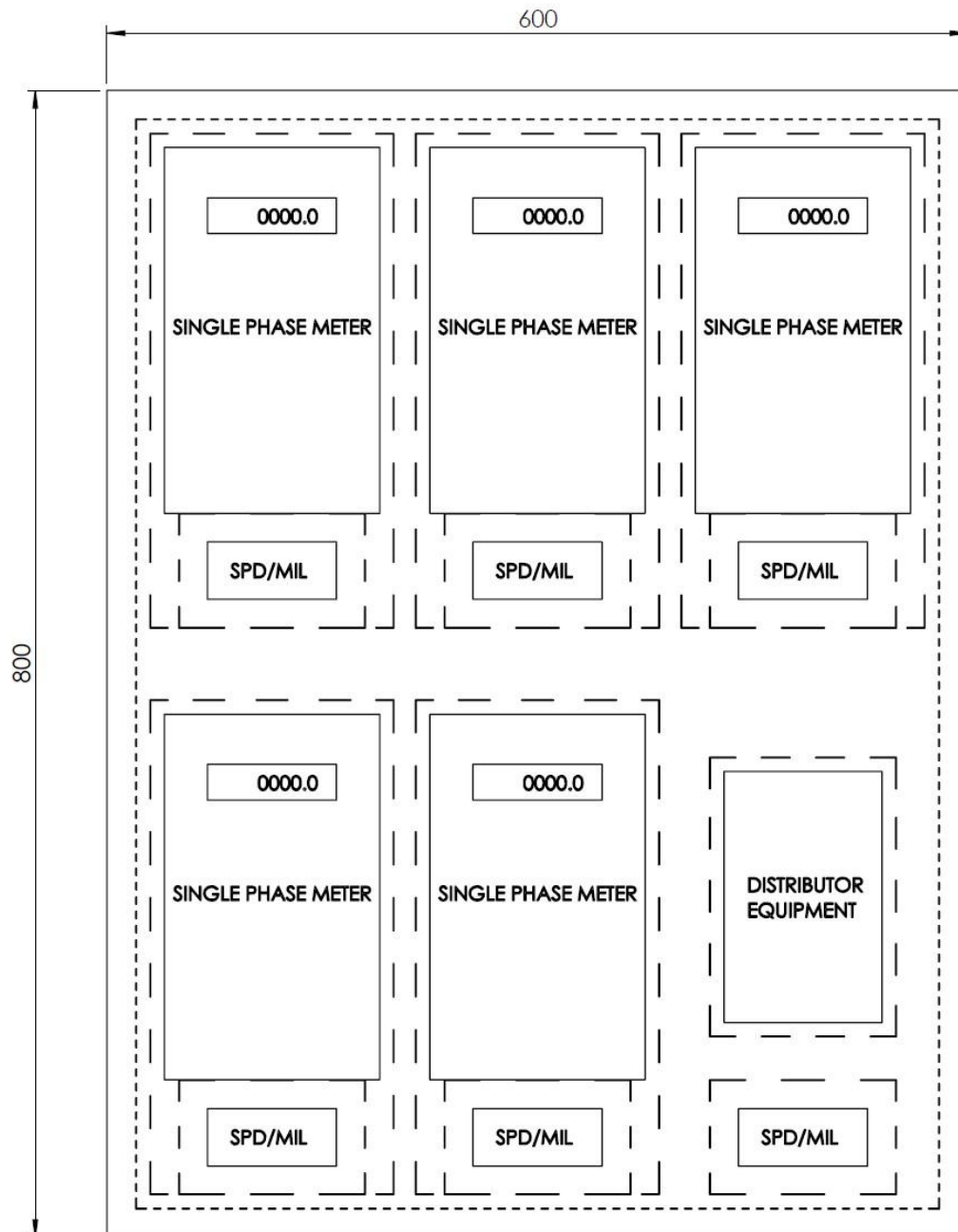
Figure 25 - Typical Panel Layout for Multi Occupancy, Single phase, 800 x 600 panel
