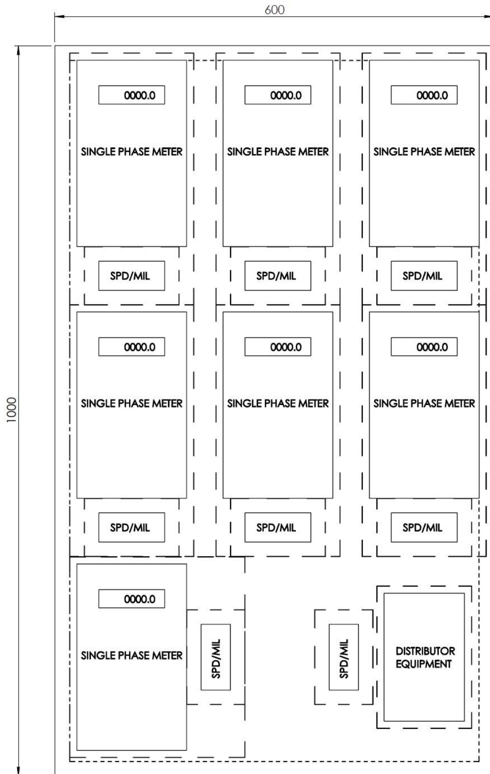
Figure 23 - Typical Panel Layout for Multi Occupancy, Single phase, 1000 x 600 panel
