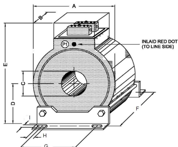
Typical Current Transformer Dimensions (Measurements in millimetres)
